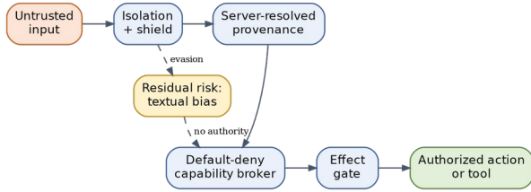
Fig. 3. Defense in depth: detection, authority, and effect containment.
